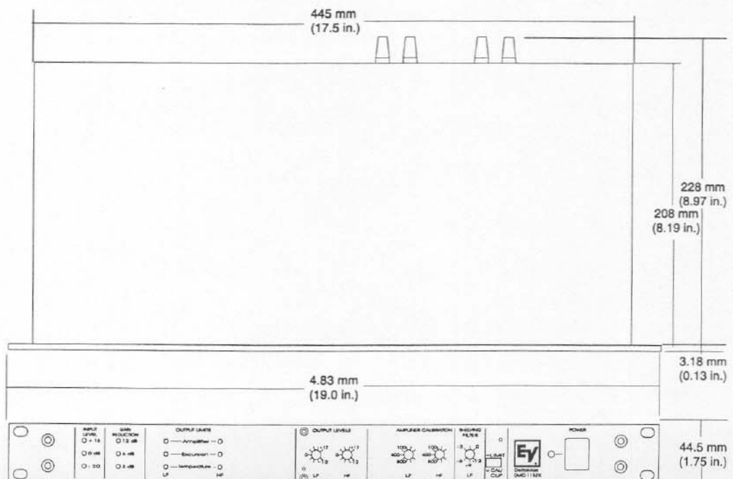
Figure 4—DMC-1152X Dimensions
